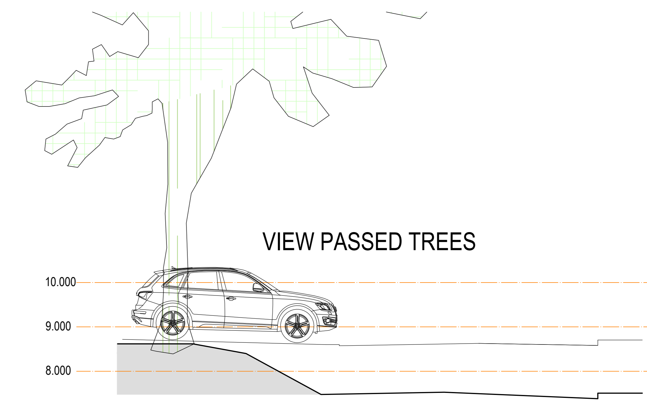
SECTION 'C'
