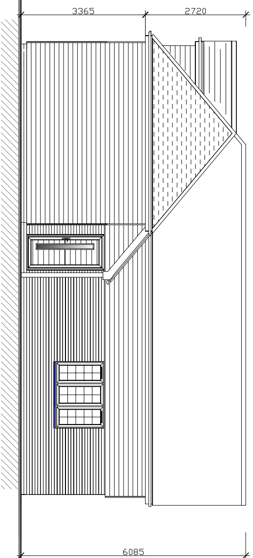
Side Elevation
