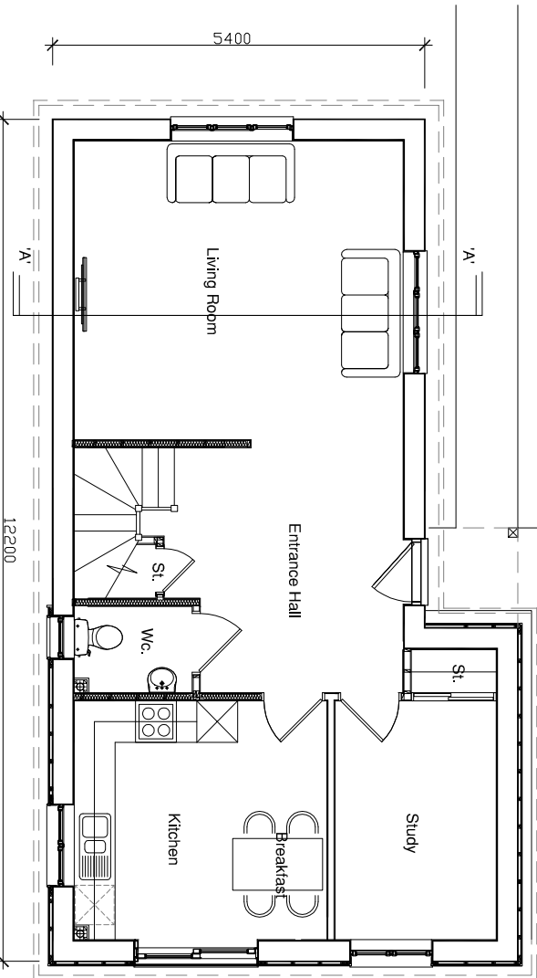
Floor Plan
