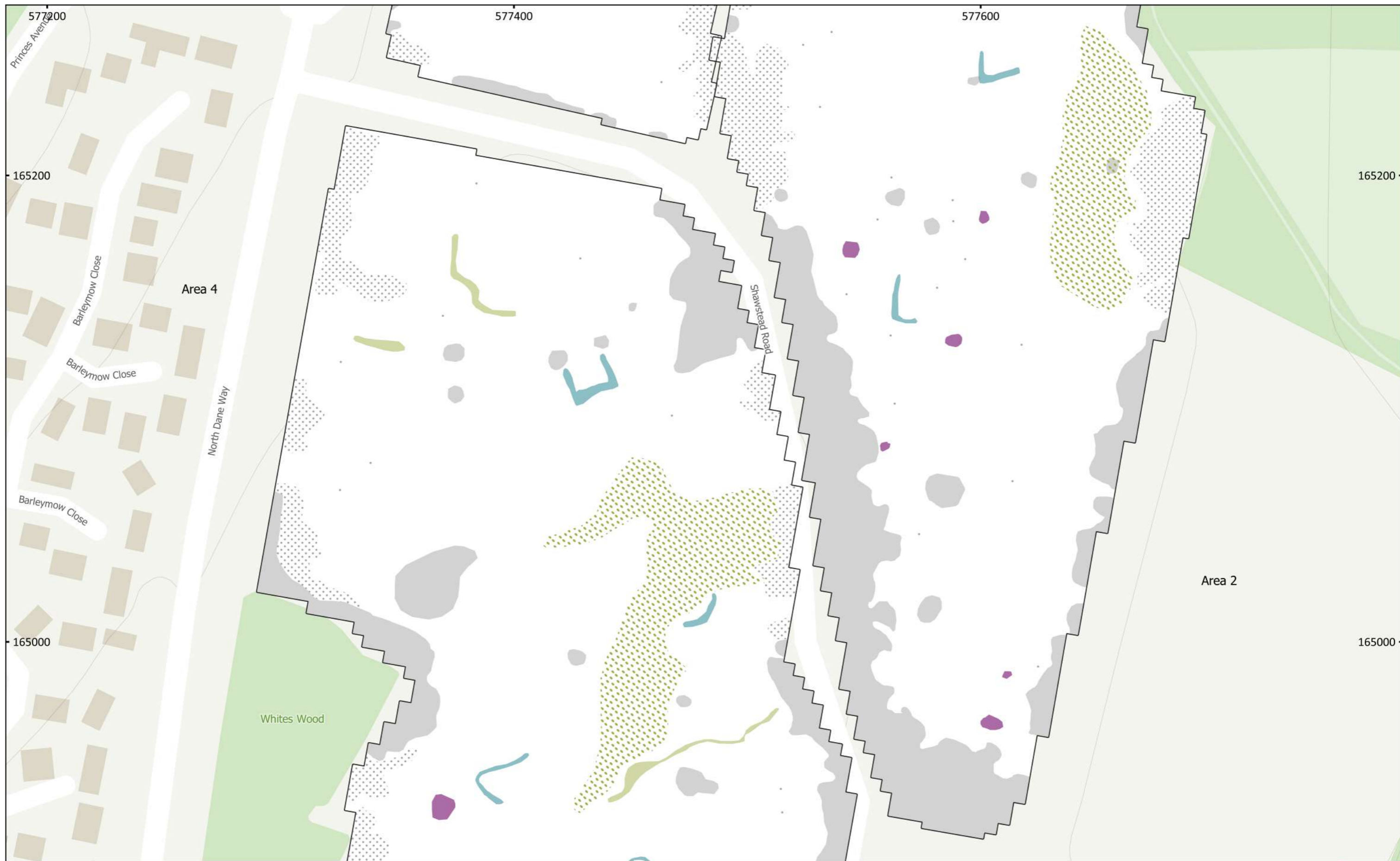
MSTQ1461 - Land at East Hill, Chatham Figure 10 - Magnetic Interpretation (Areas 2, 3 & 4) 1:1,500 @ A3 Copyright Magnitude Surveys Ltd 2022 Contains Ordnance Survey data © Crown Copyright and database right 2022
