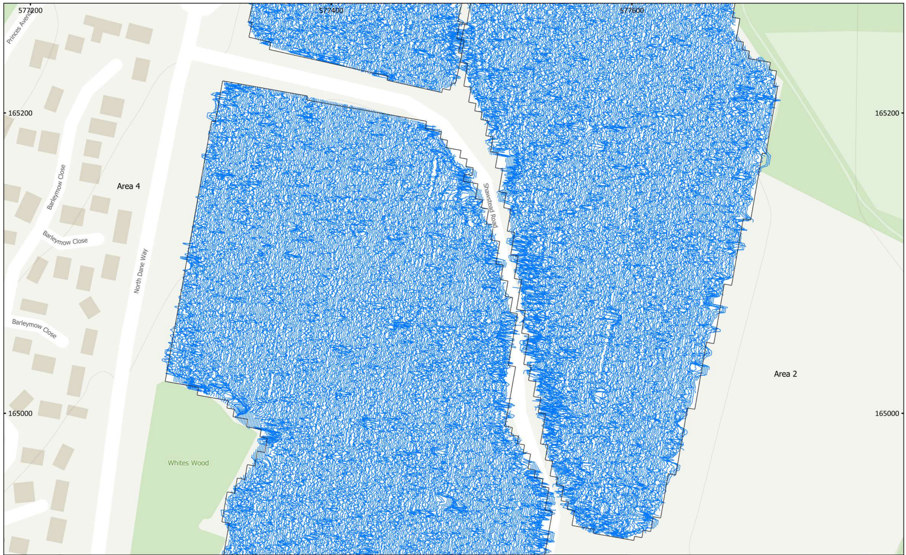
MSTQ1461 - Land at East Hill, Chatham Figure 11 - XY Trace Plot (Areas 2, 3 & 4) 30nT/cm at 1:1,500 @ A3 Copyright Magnitude Surveys Ltd 2022 Contains Ordnance Survey data © Crown Copyright and database right 2022
