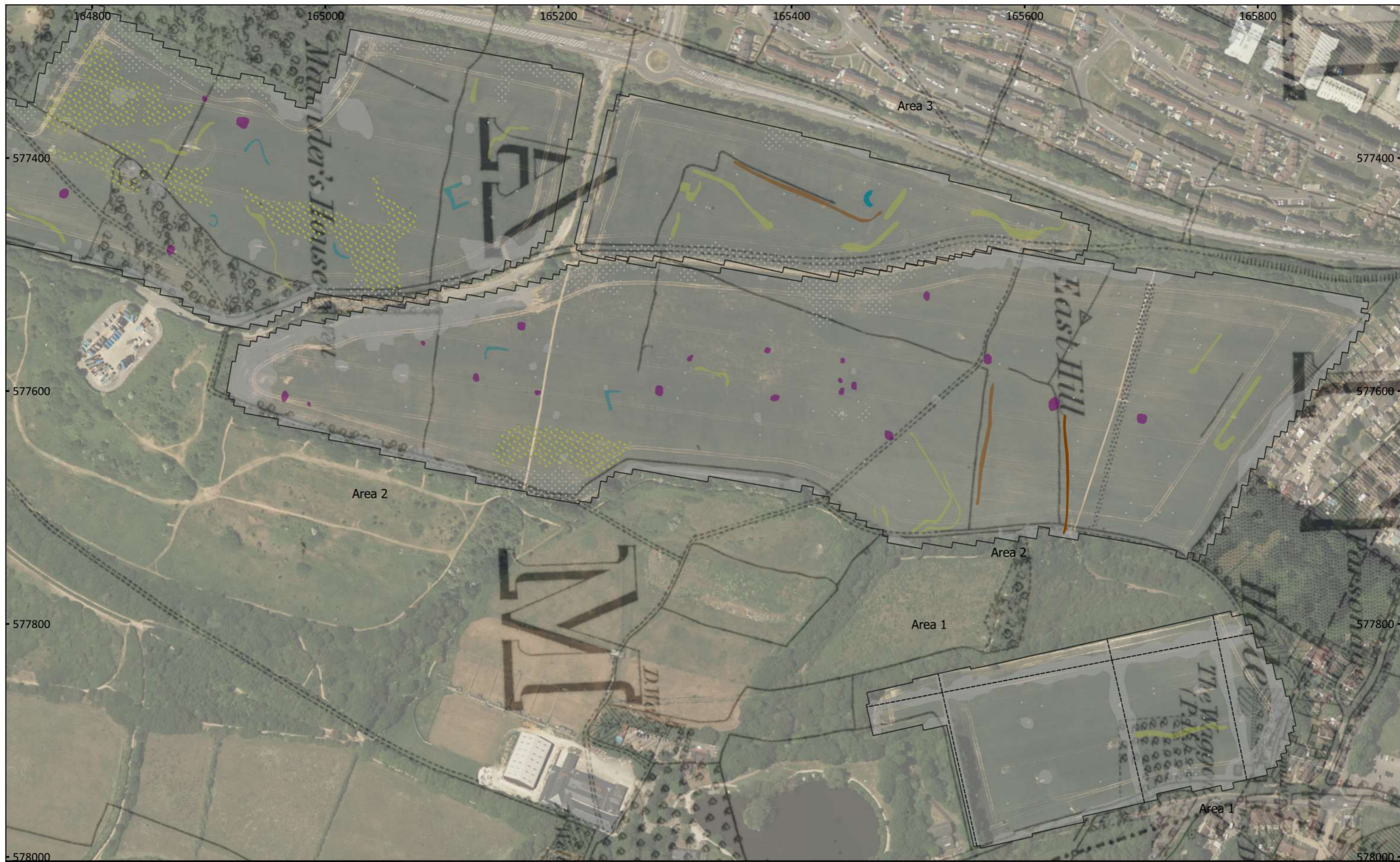
MSTQ1461 - Land at East Hill, Chatham Figure 18 - Magnetic Interpretation Over Historical Maps and Satellite Imagery (Areas 1, 2, 3 & 4) 1:3,000 @ A3 Copyright Magnitude Surveys Ltd 2022 Contains historical mapping © CLS Data 2022: Ordnance Survey, 6" 2nd edition c. 1882-1913 Contains satellite imagery © Bing Satellite 2022
