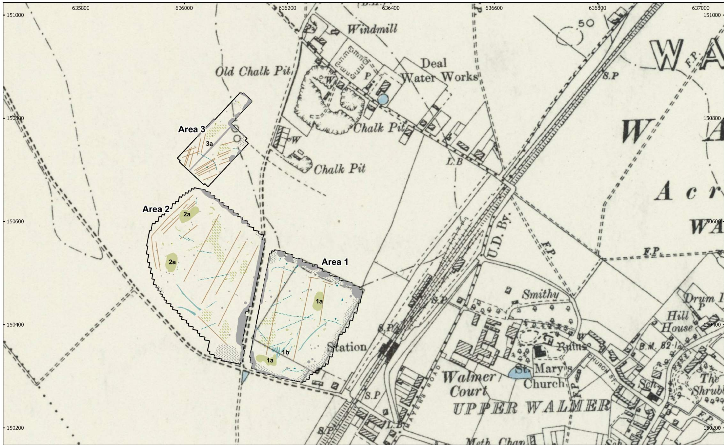
MSTR121 - Land at Cross Road, Deal, Kent Figure 6 - Magnetic Interpretation over Historic Mapping 1:3500 @ A3 Copyright Magnitude Surveys Ltd 2017 Contains historic mapping: Ordnance Survey, 6" 2nd edition c. 1882-1913 © National Library of Scotland
