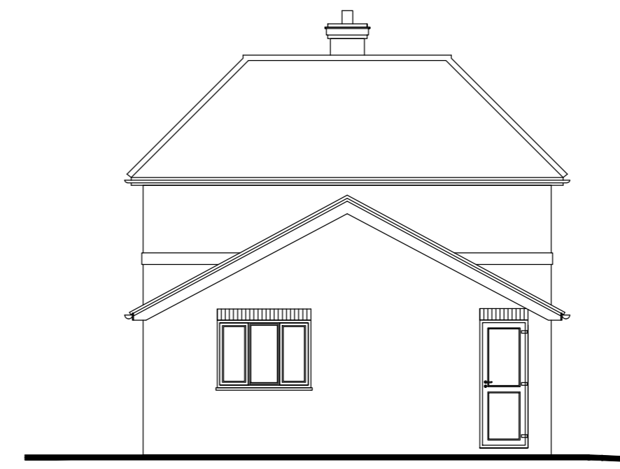
North Elevation as Proposed 1:100
