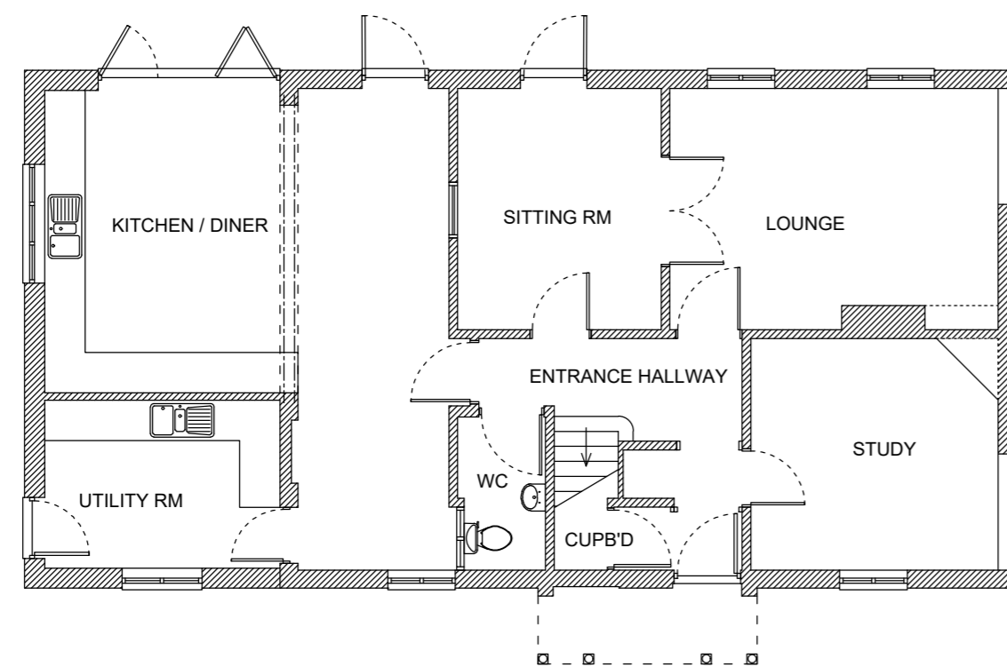
Ground Floor Plan as Proposed 1:100
