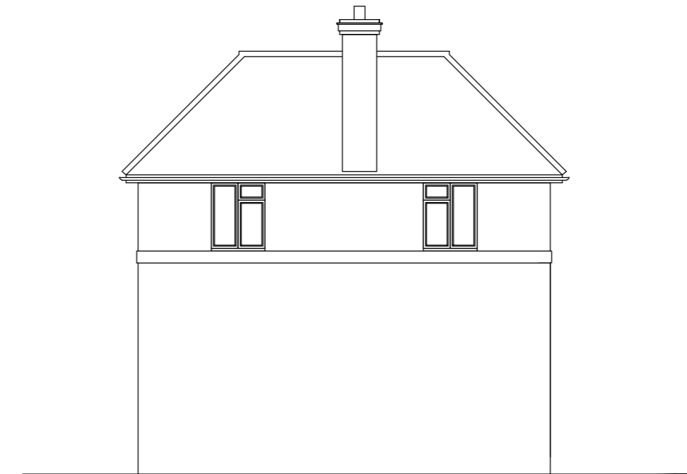
South Elevation as Proposed 1:100
