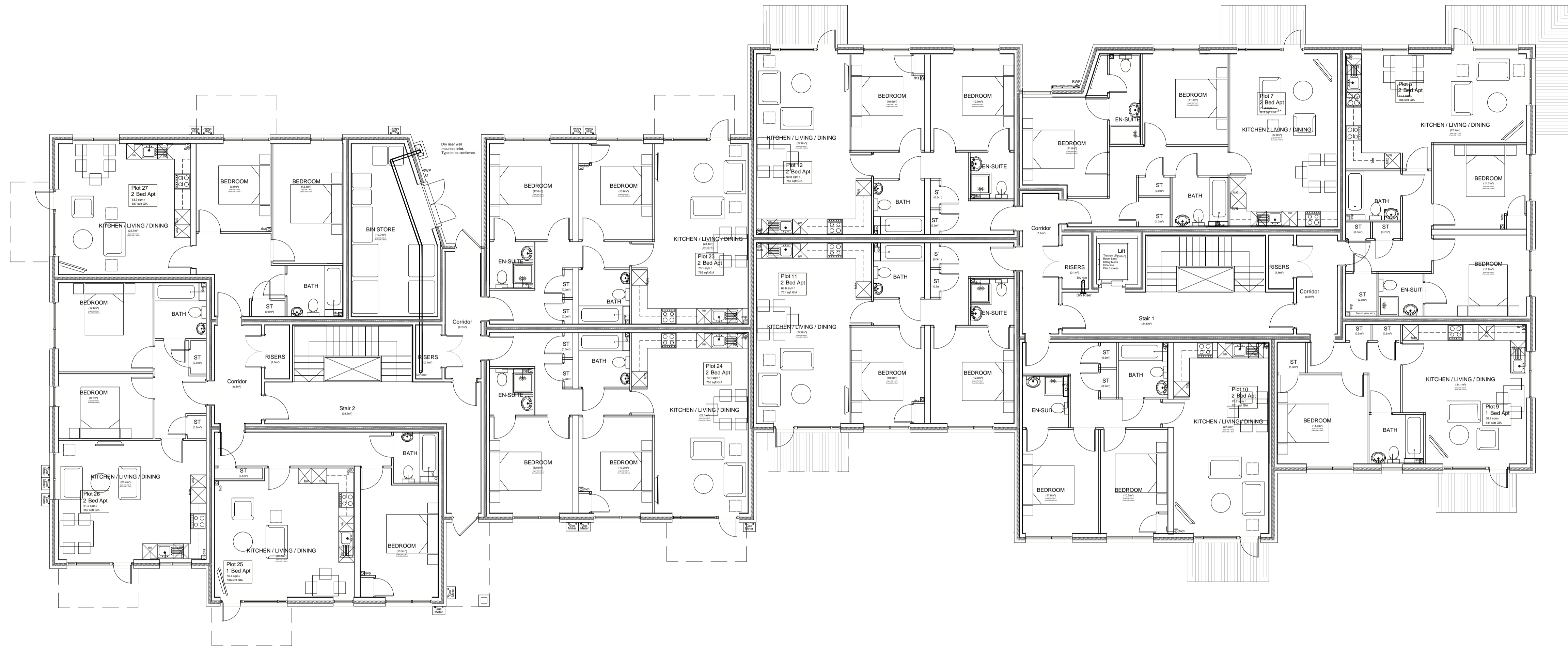
Upper Ground Floor GIA (894.9m 2 )
