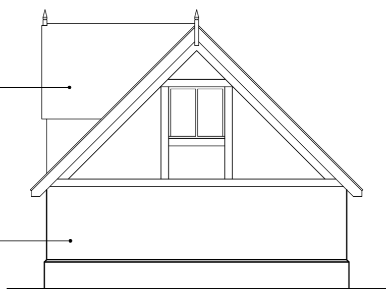
Side (North) Elevation Z
